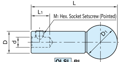
QLSL-RL (Plug-In Handles)
