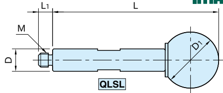
QLSL (Screw-In Handles)
